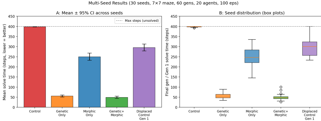
Figure 2: Multi-seed results: mean \pm 95% CI (left, bar chart) and distribution across 30 seeds (right, box plots) for all conditions. The displaced control Gen 1 column is the headline result.
