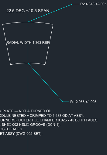
VIEW A — RADIAL PROFILE (DEPLOYED GEOMETRY) SCALE 1.2:1
