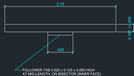
VIEW B — AXIAL SECTION SCALE 1.6:1
