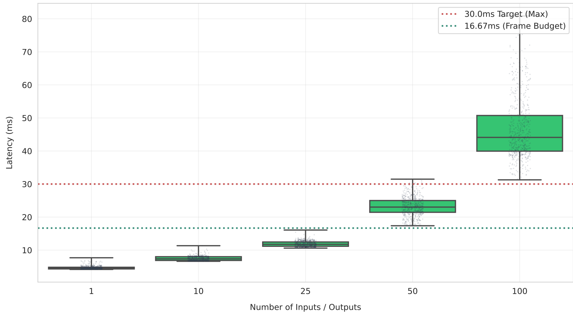
Cross-Layer Pipeline Latency Distribution by Configuration
