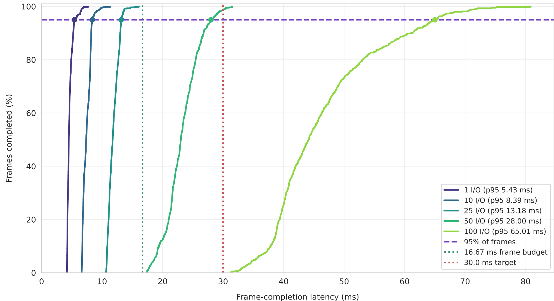
Cross-Layer Pipeline Frame-Completion Latency Distribution
