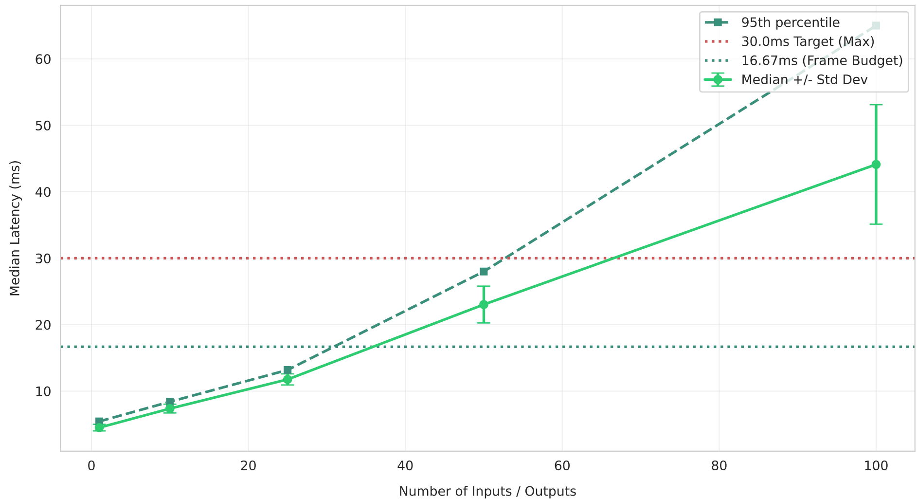
Cross-Layer Pipeline Latency vs I/O Count
