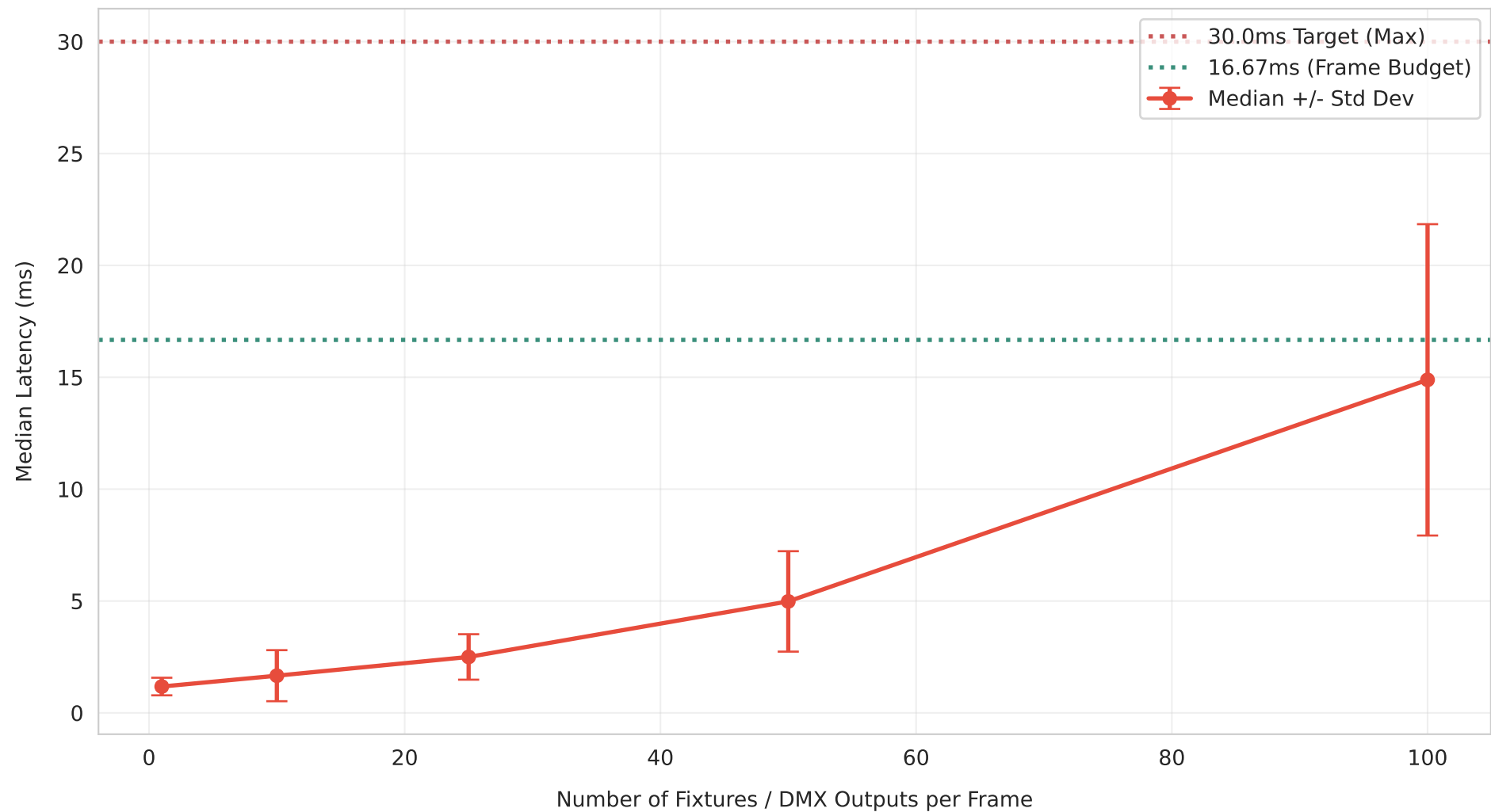
Fixture Layer Latency vs Input Count
