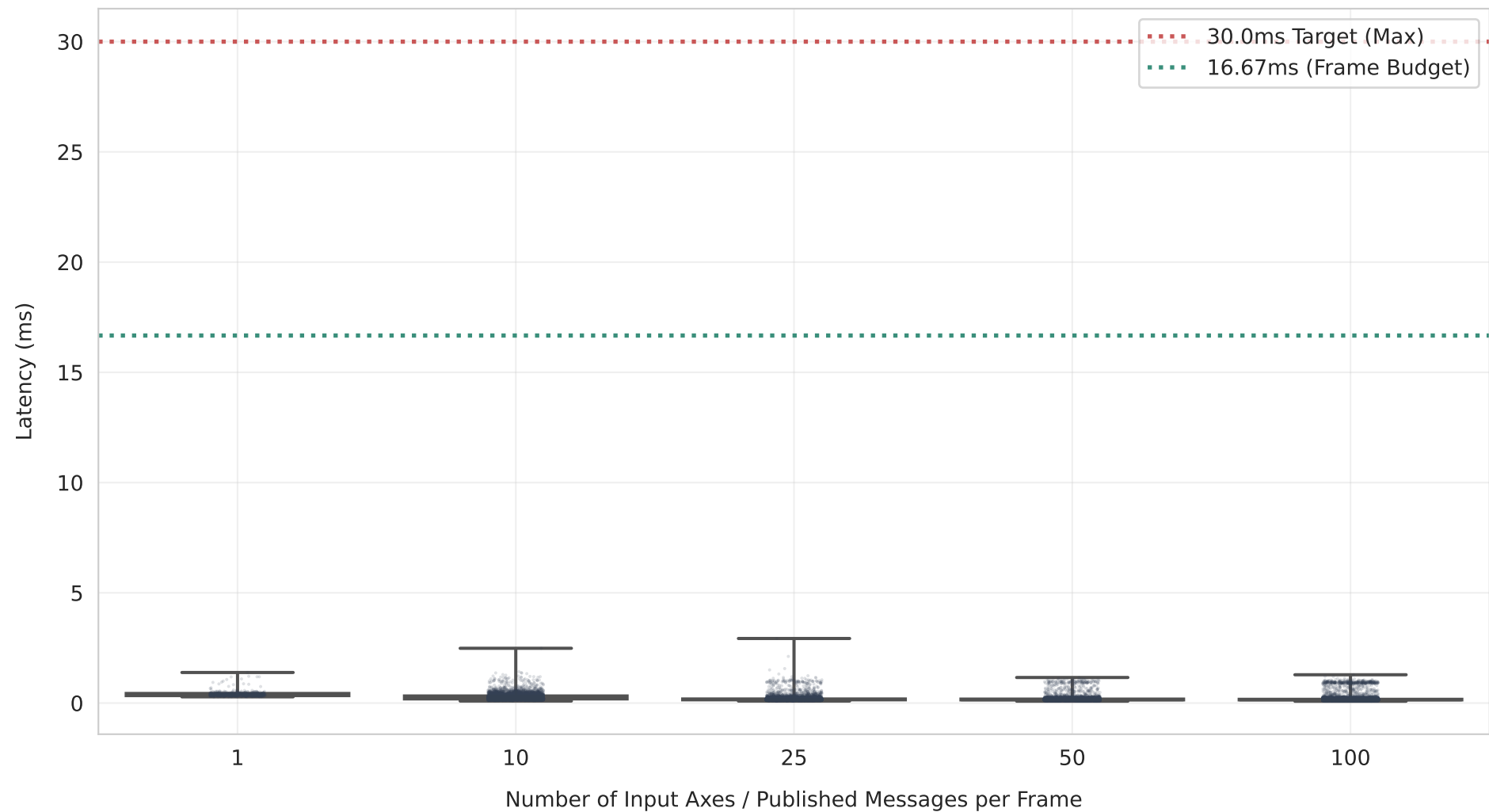
Input Layer Latency Distribution by Configuration
