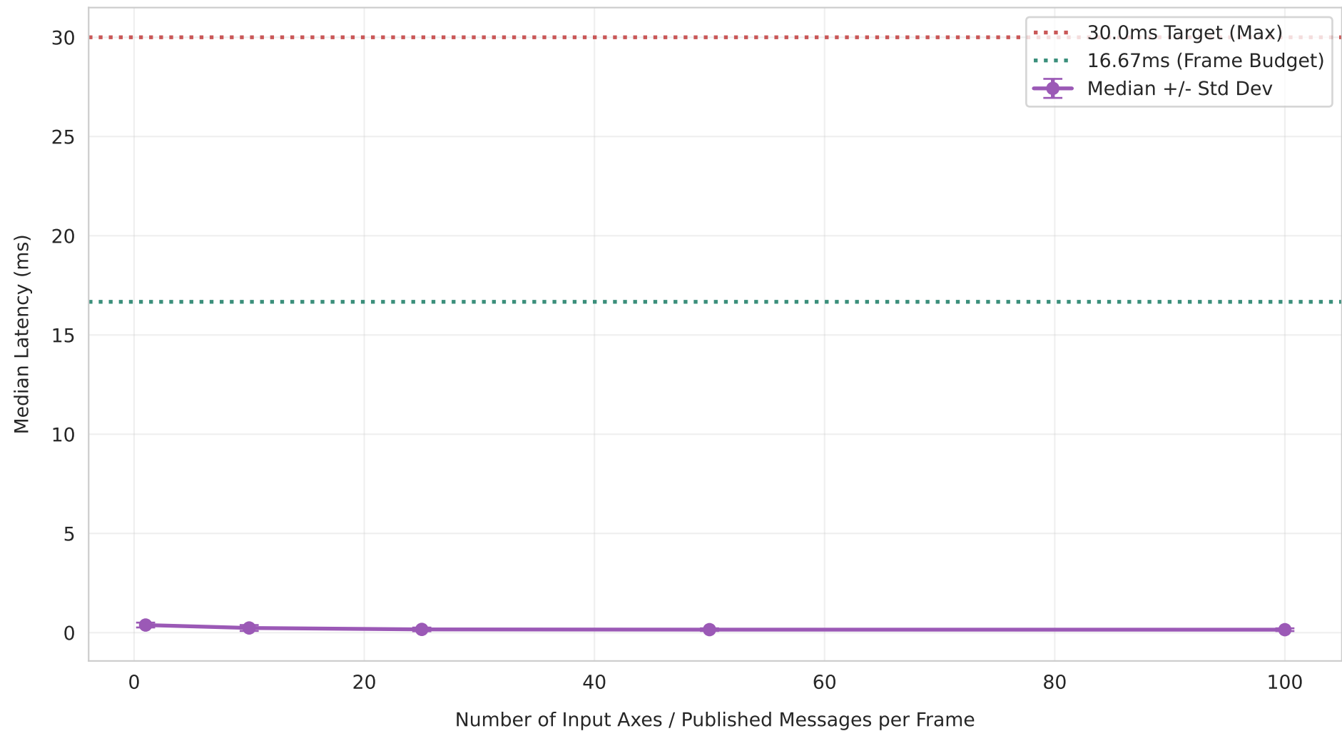
Input Layer Latency vs Input Count
