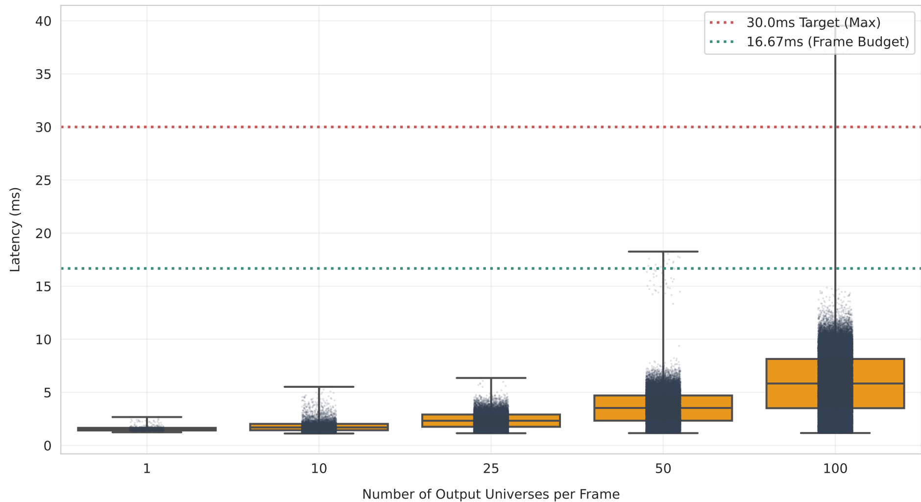
Output Layer Latency Distribution by Configuration
