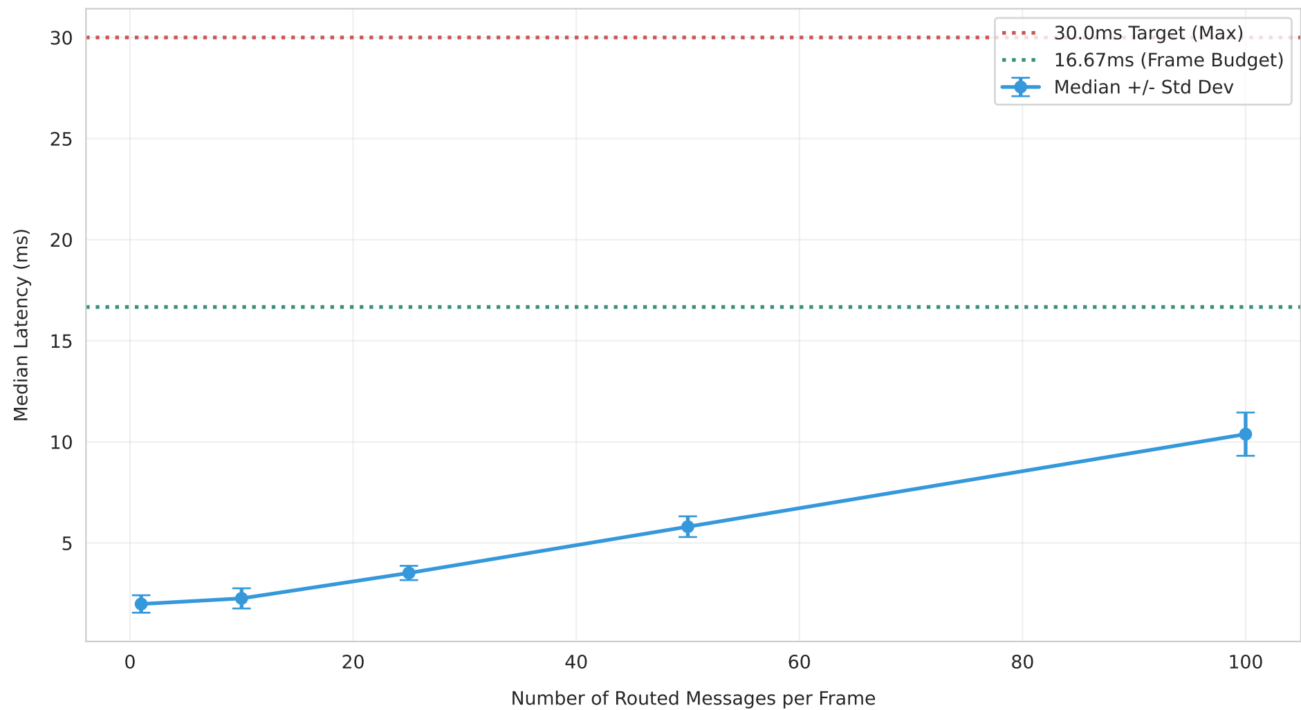
Router Layer Latency vs Input Count
