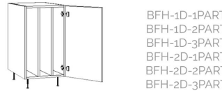
Base Cabinet, 1 Door 24-66" W
