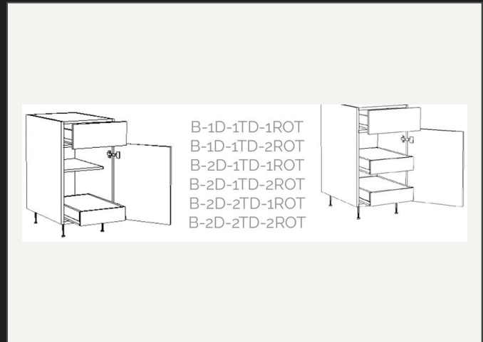
Base Cabinet, 1 Door + 1 Drawer 24-42" W - 6 configurations
