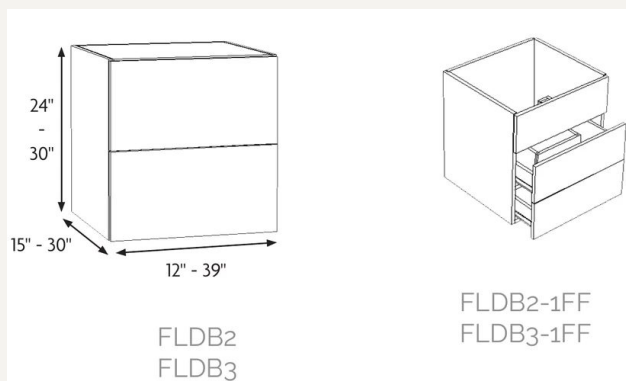
Base Cabinet
