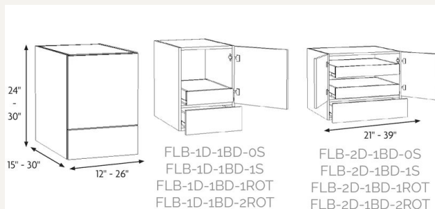
Base Cabinet, 1 Door + 1 Drawer
