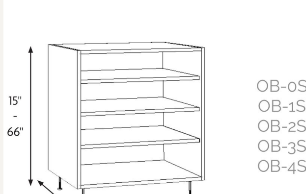
Base Cabinet
