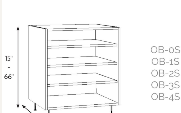
Base Cabinet
