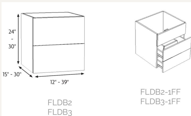
Base Cabinet
