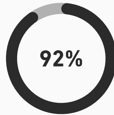
Service UI
