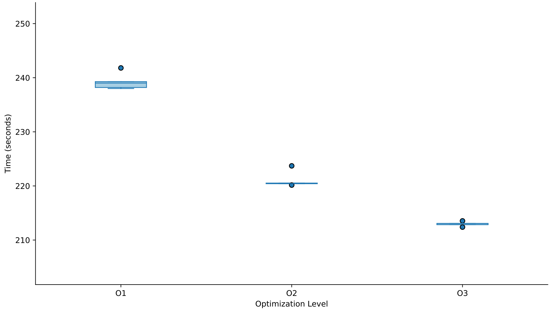
Execution Time for 641
