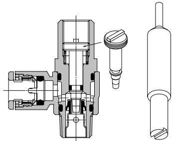
Special tool Part number: AS-T-1
