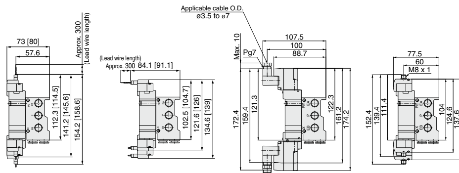
M8 connector (WO)
