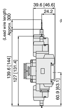
L plug connector (L)
