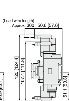
M plug connector (M)
