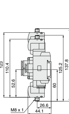
M8 connector (WO)
