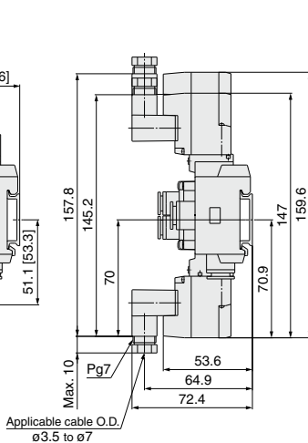
M plug connector (M)
