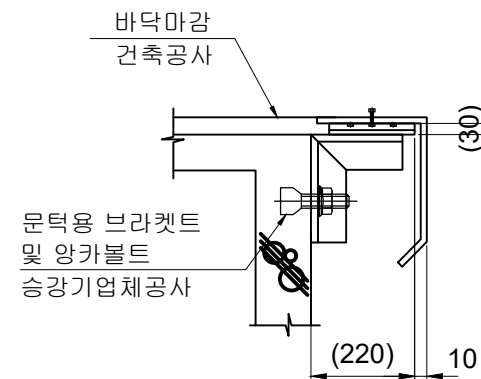
SEC "X-X"
