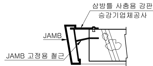
SEC "A-A"
