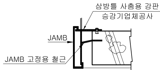
SEC "B-B"
