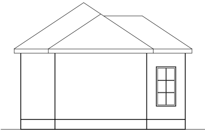
Left Elevation
