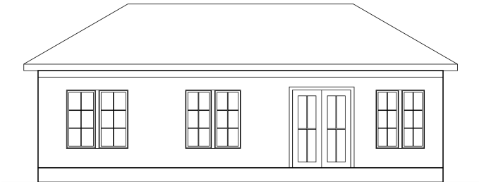
Back Elevation
