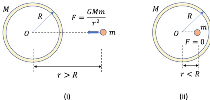
Figure: Shell theorem for (i) r > R and (ii) r < R respectively.
