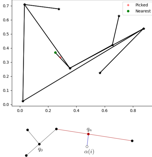
Figure 5.18: If the nearest point in S lies in an edge, then the edge is split into two, and a new vertex is inserted into \mathcal{G} .
