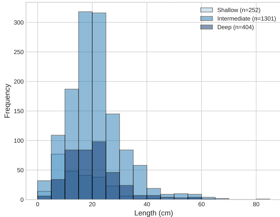
Size Distribution by Depth (5 cm bins)
