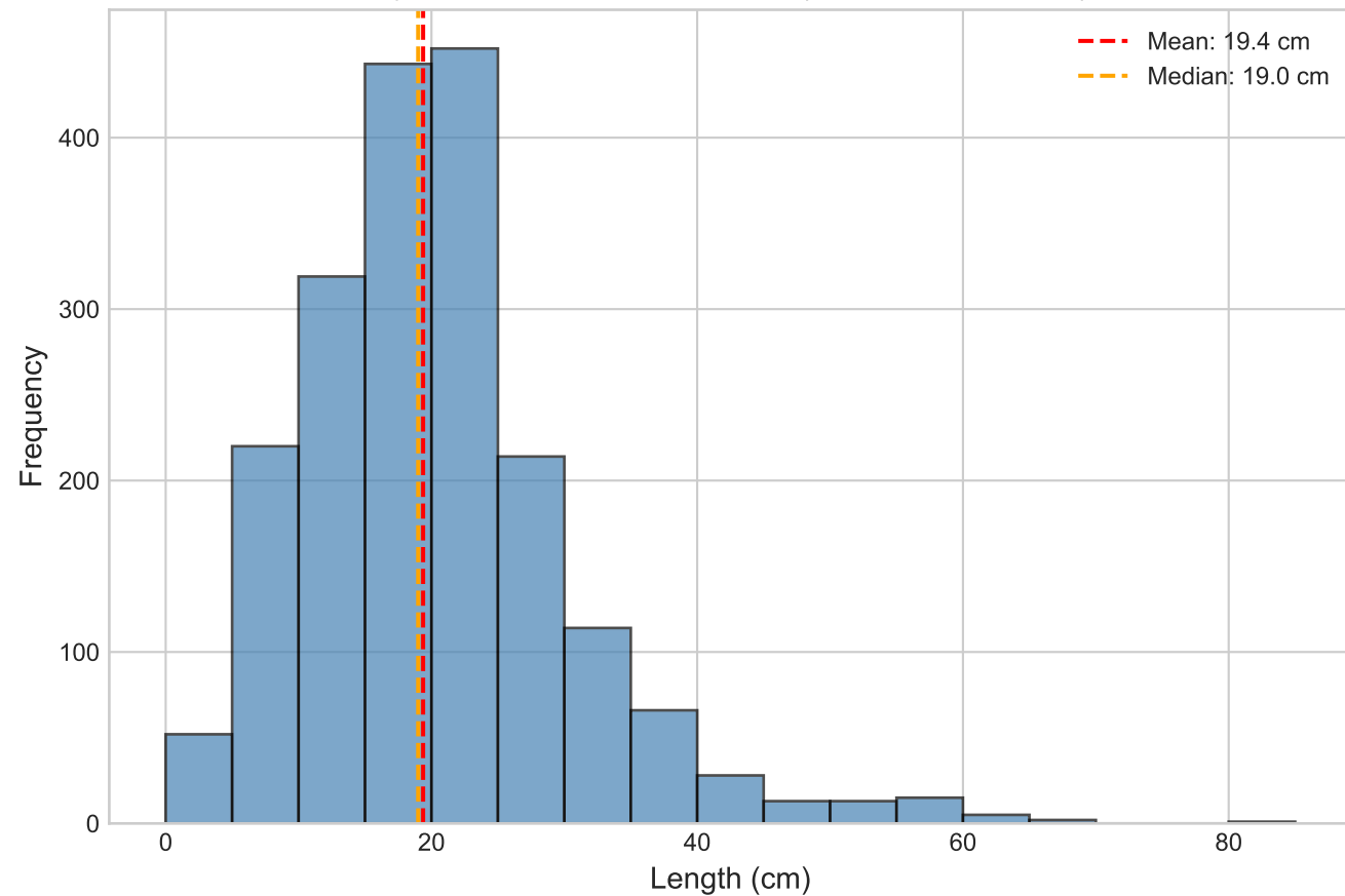
Pycnopodia Size Distribution (5 cm bins, n=1957)
