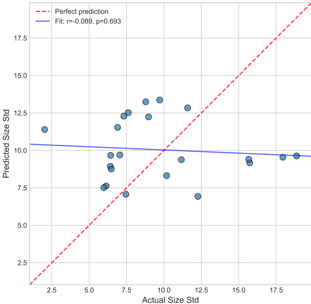
Random Forest: Predicted vs Actual Size Std
