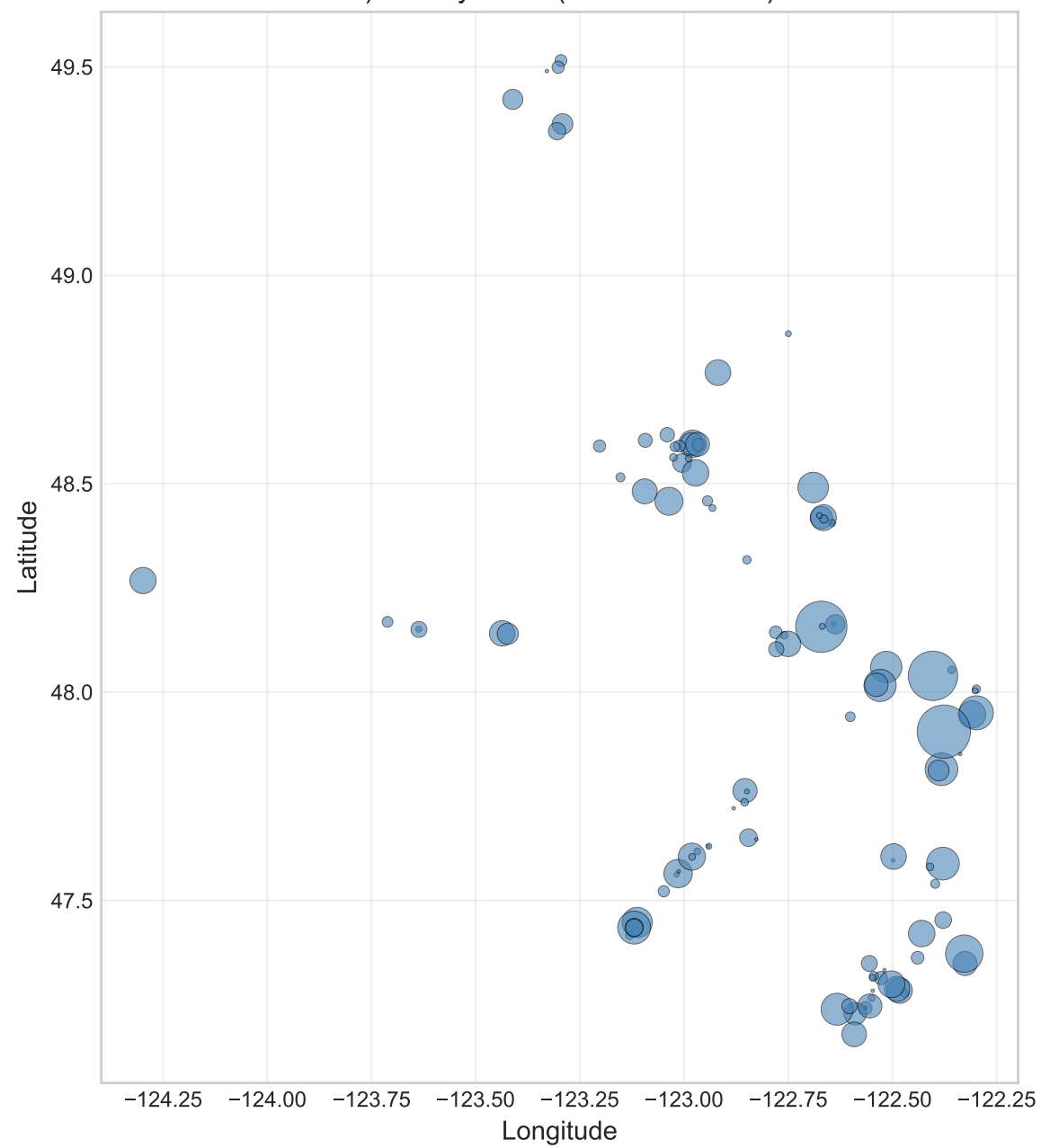
C) Survey Effort (size = transects)
