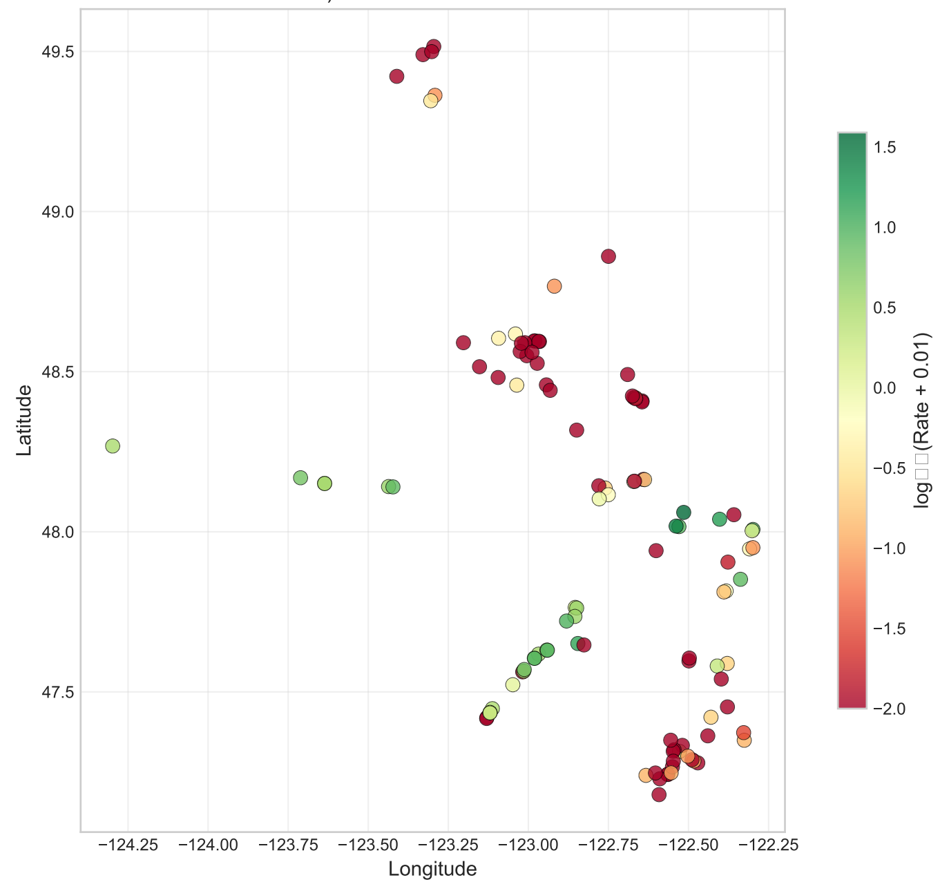
D) Mean Encounter Rate
