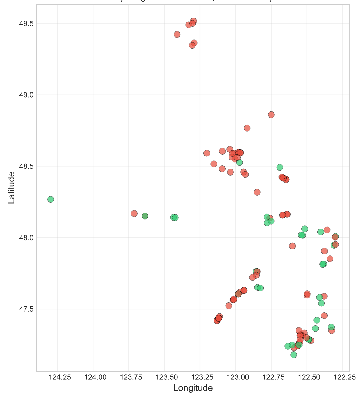
D) Mean Encounter Rate
