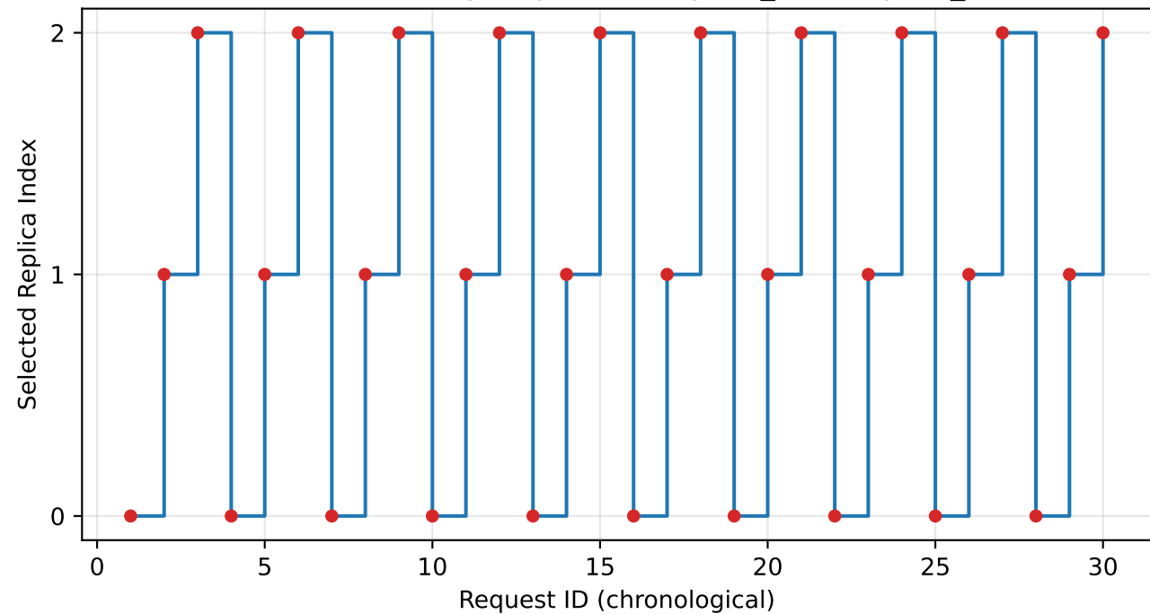
Round-Robin Routing Sequence (request_id -> replica_index)
