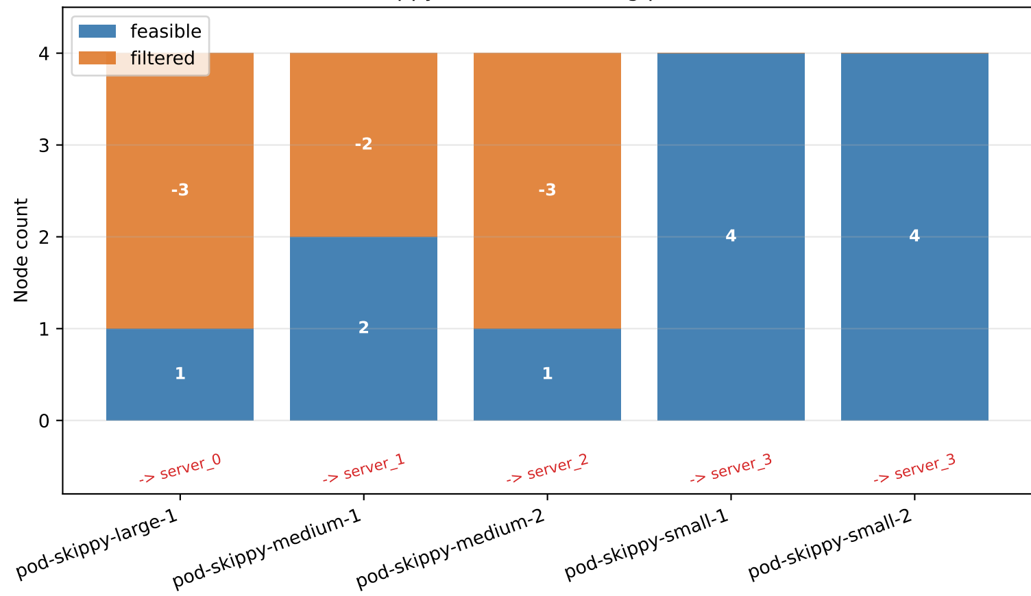
Skippy Resource Filtering per Pod
