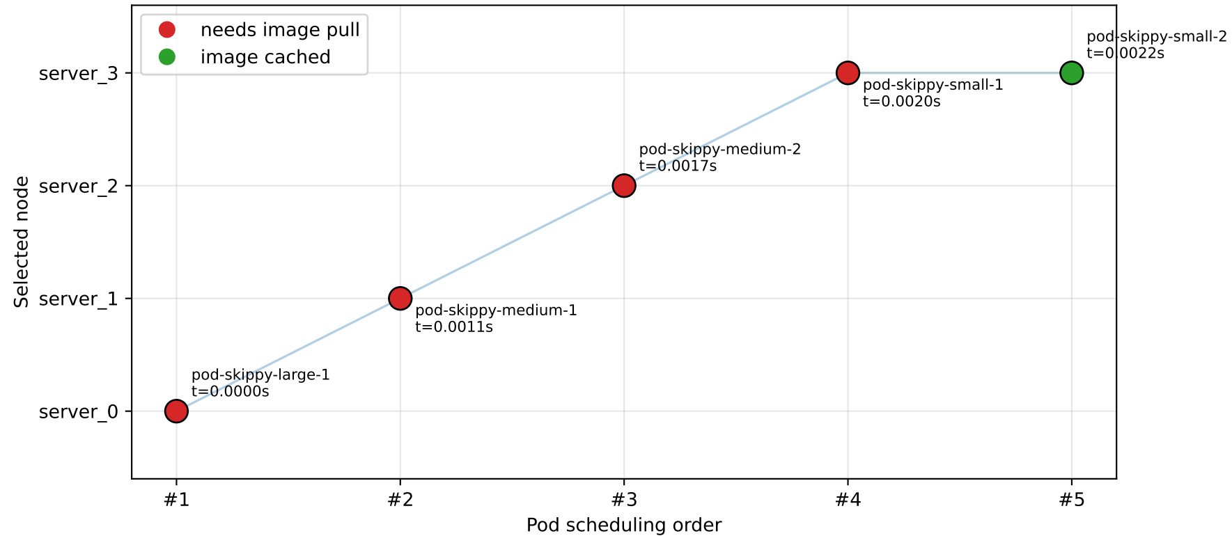
Skippy Scheduling Order and Selected Node
