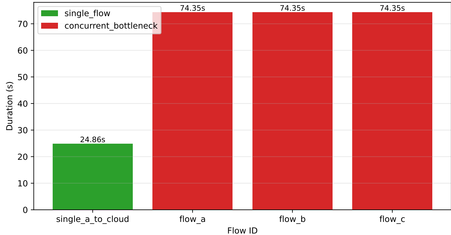
Per-Flow Duration: single vs concurrent bottleneck
