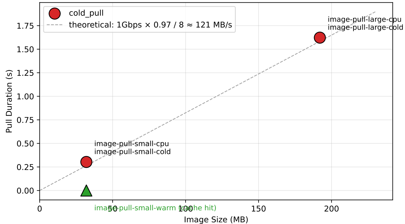
Image Pull Duration vs Image Size (Skippy + docker.pull)
