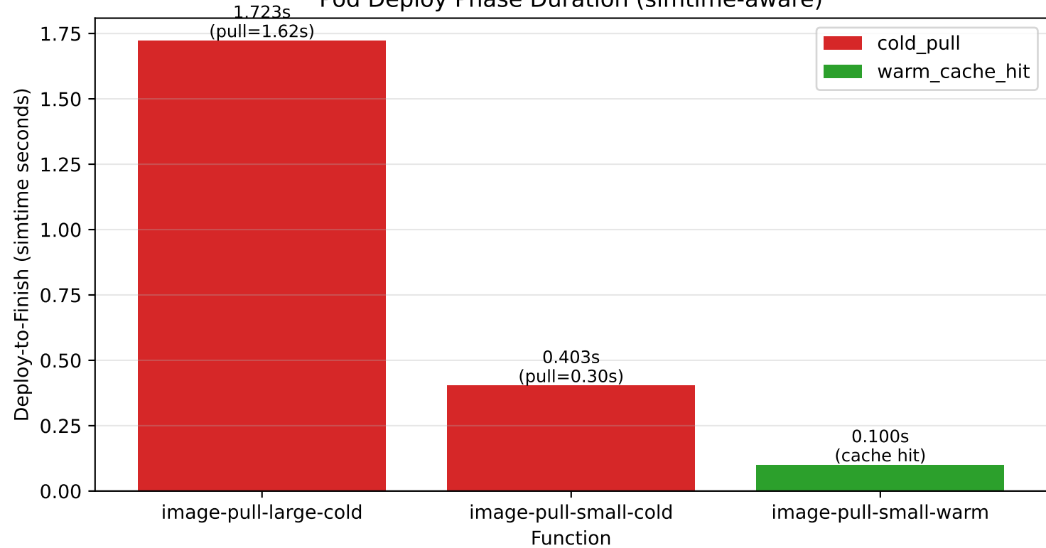
Pod Deploy Phase Duration (simtime-aware)
