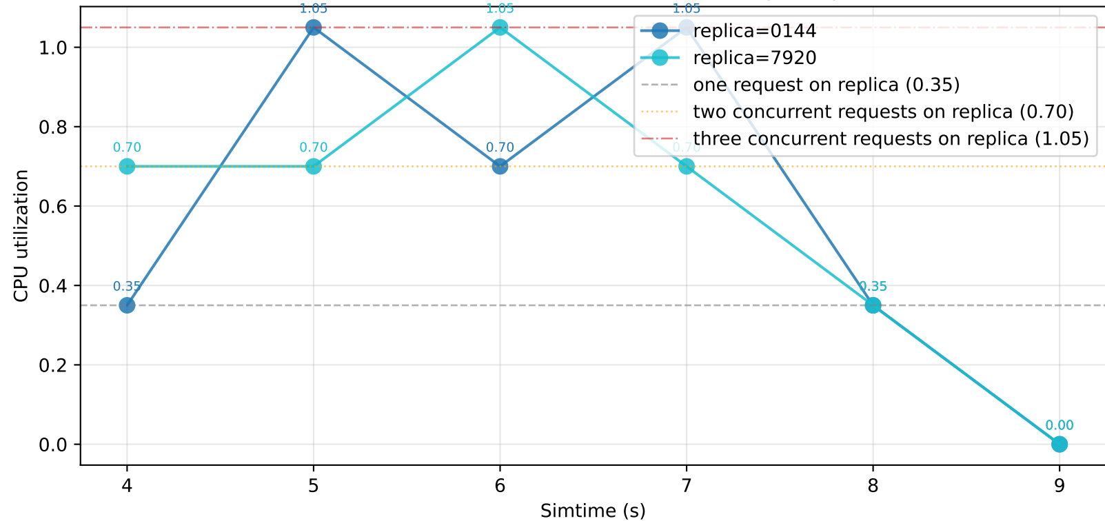
ResourceMonitor CPU Utilization Timeline (per-replica)
