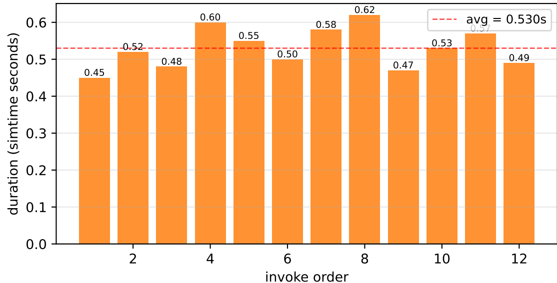
trace-slow-python-pi (avg=0.530s, n=12)
