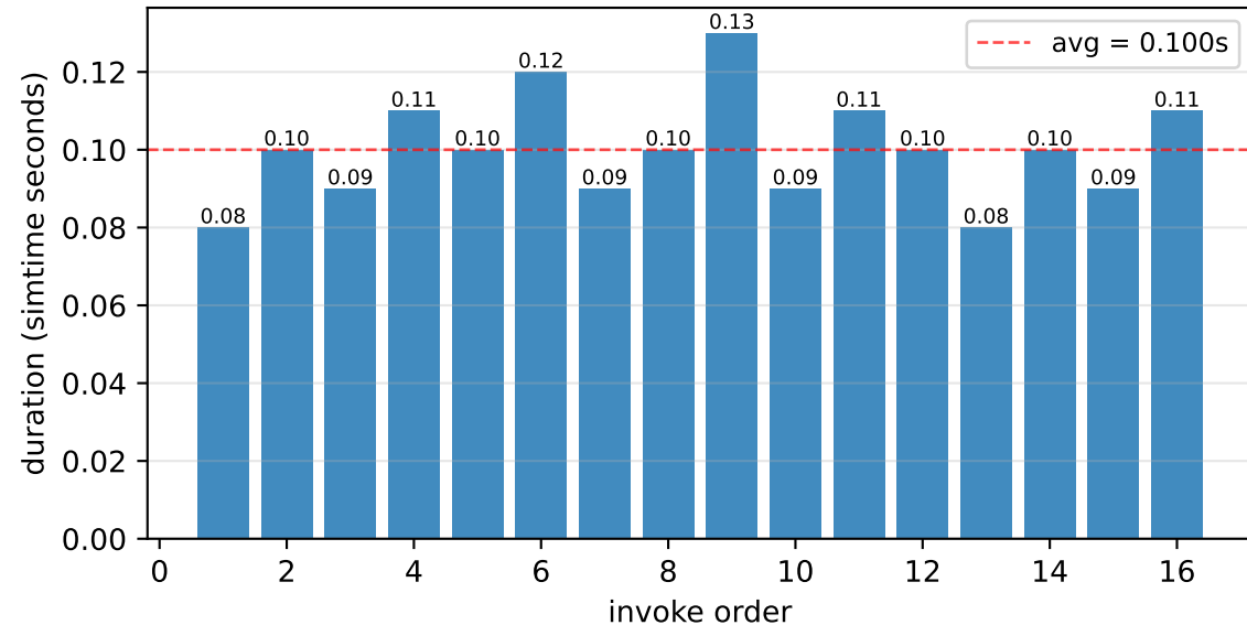
trace-fast-python-pi (avg=0.100s, n=16)
