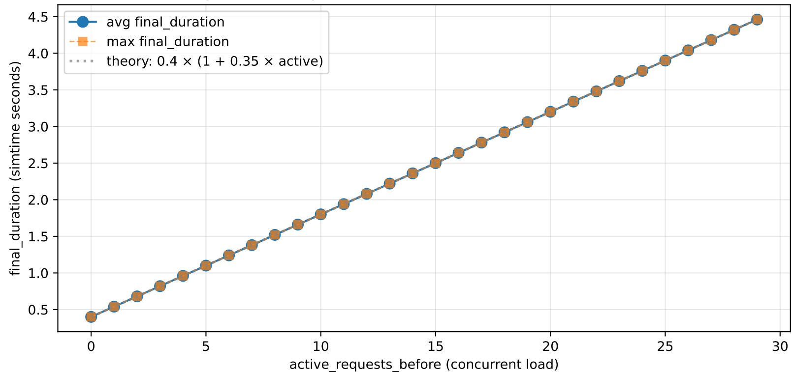
Degradation: request execution time vs node concurrent load
