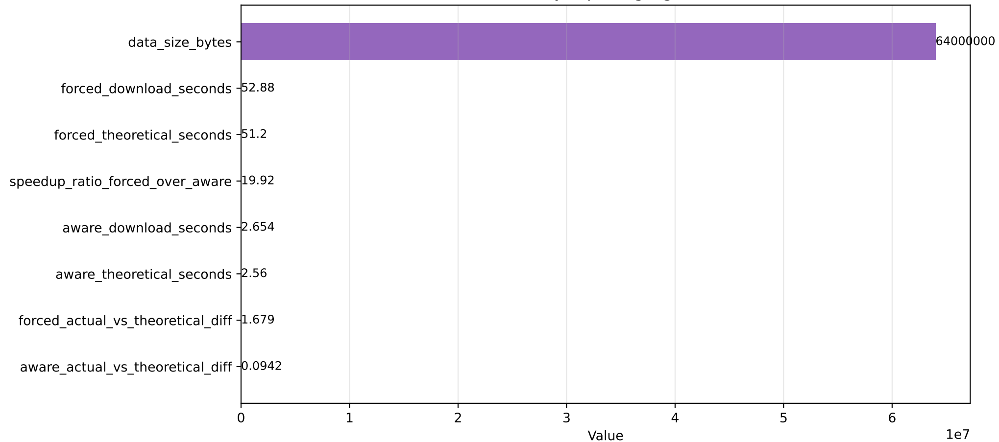
Data Locality Paper Highlight Metrics
