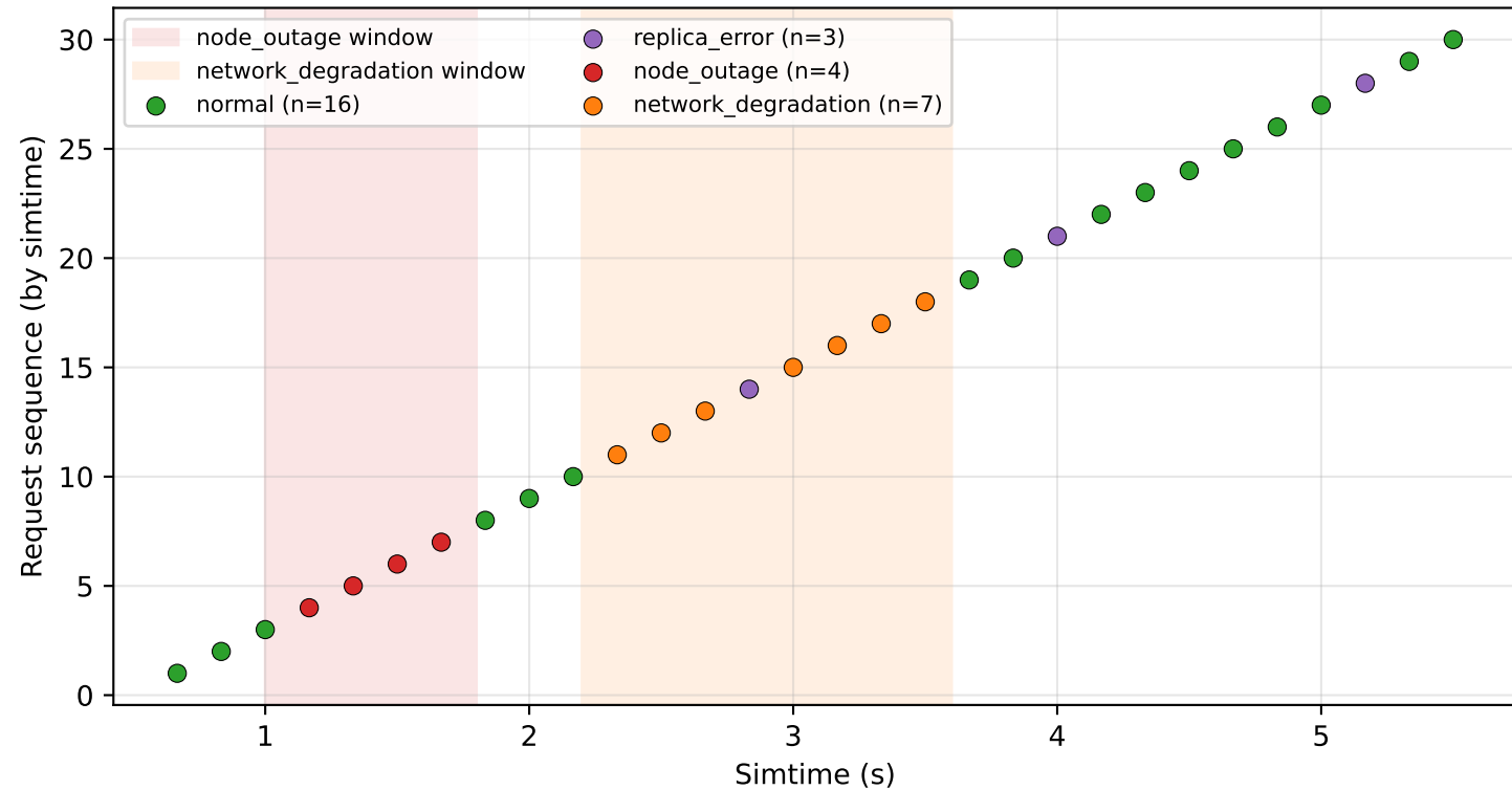
Request Timeline vs Fault Windows (server_0)
