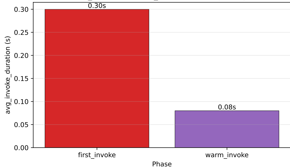
first_invoke vs warm_invoke (3.75x speedup)
