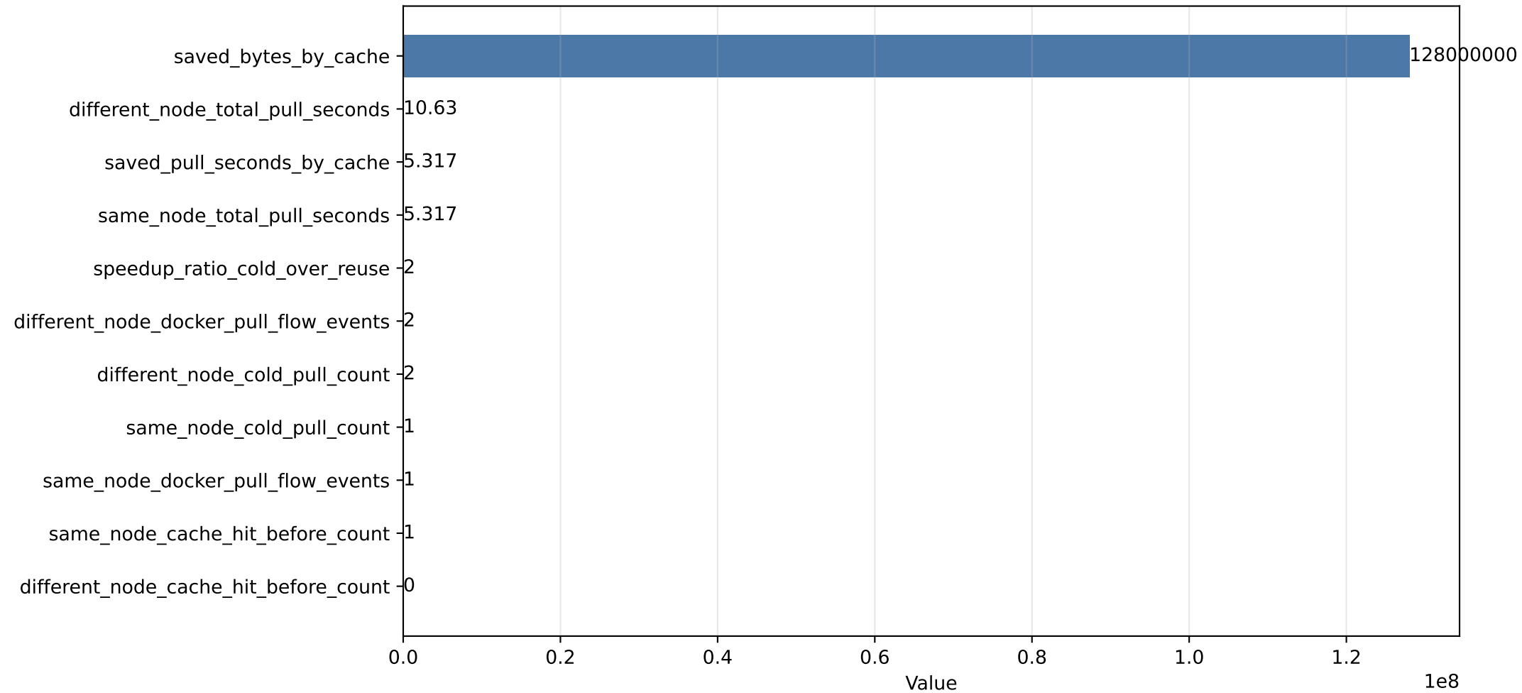
Image Cache Paper Highlight Metrics
