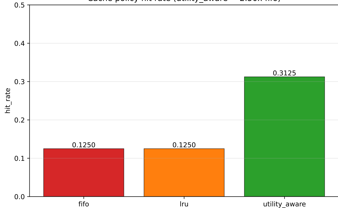
Cache policy hit rate (utility_aware = 2.50x fifo)
