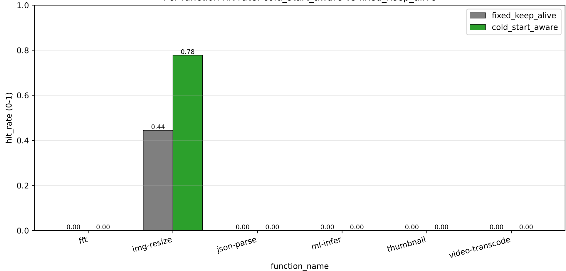
Per-function hit rate: cold_start_aware vs fixed_keep_alive
