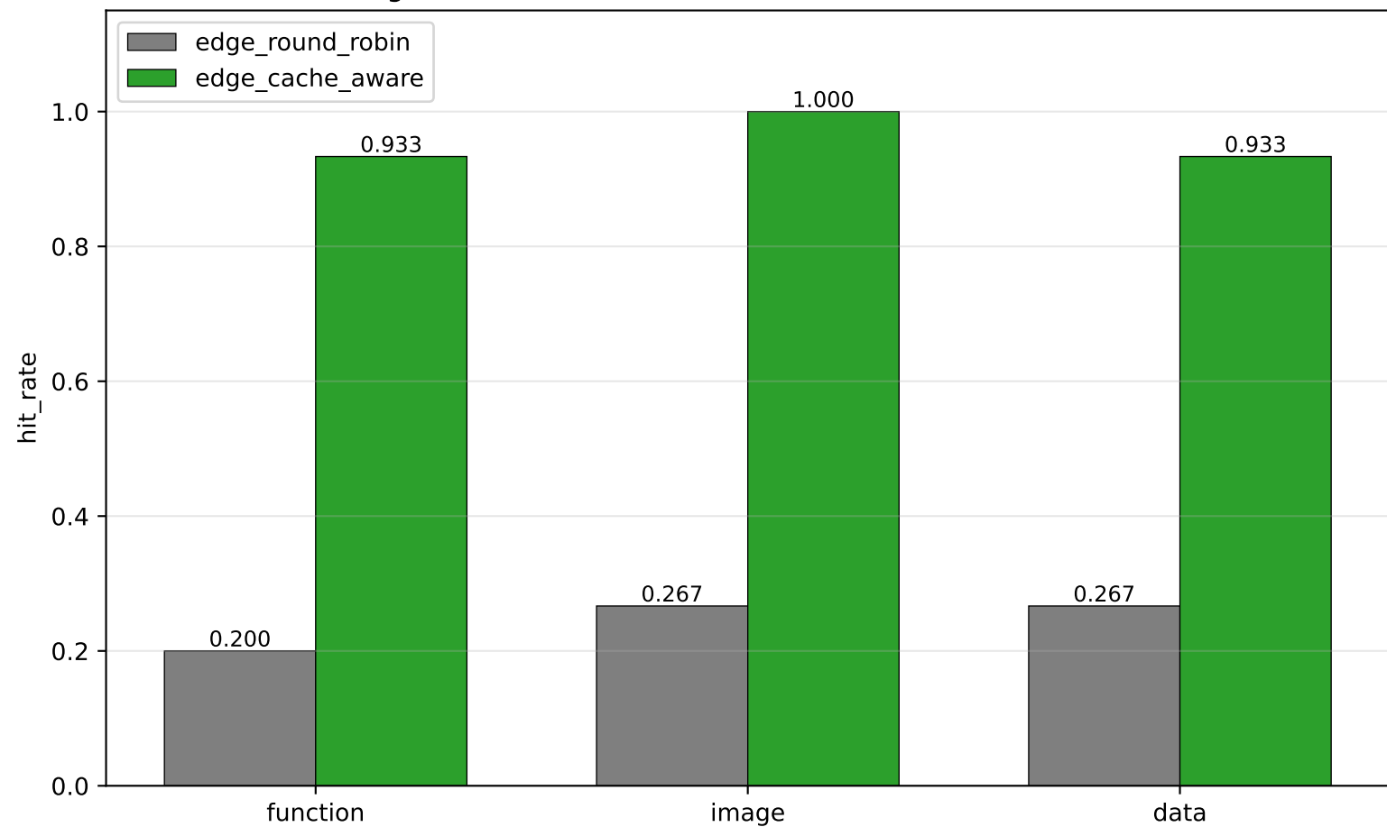
Edge cache scheduler: three cache dimension hit rates
