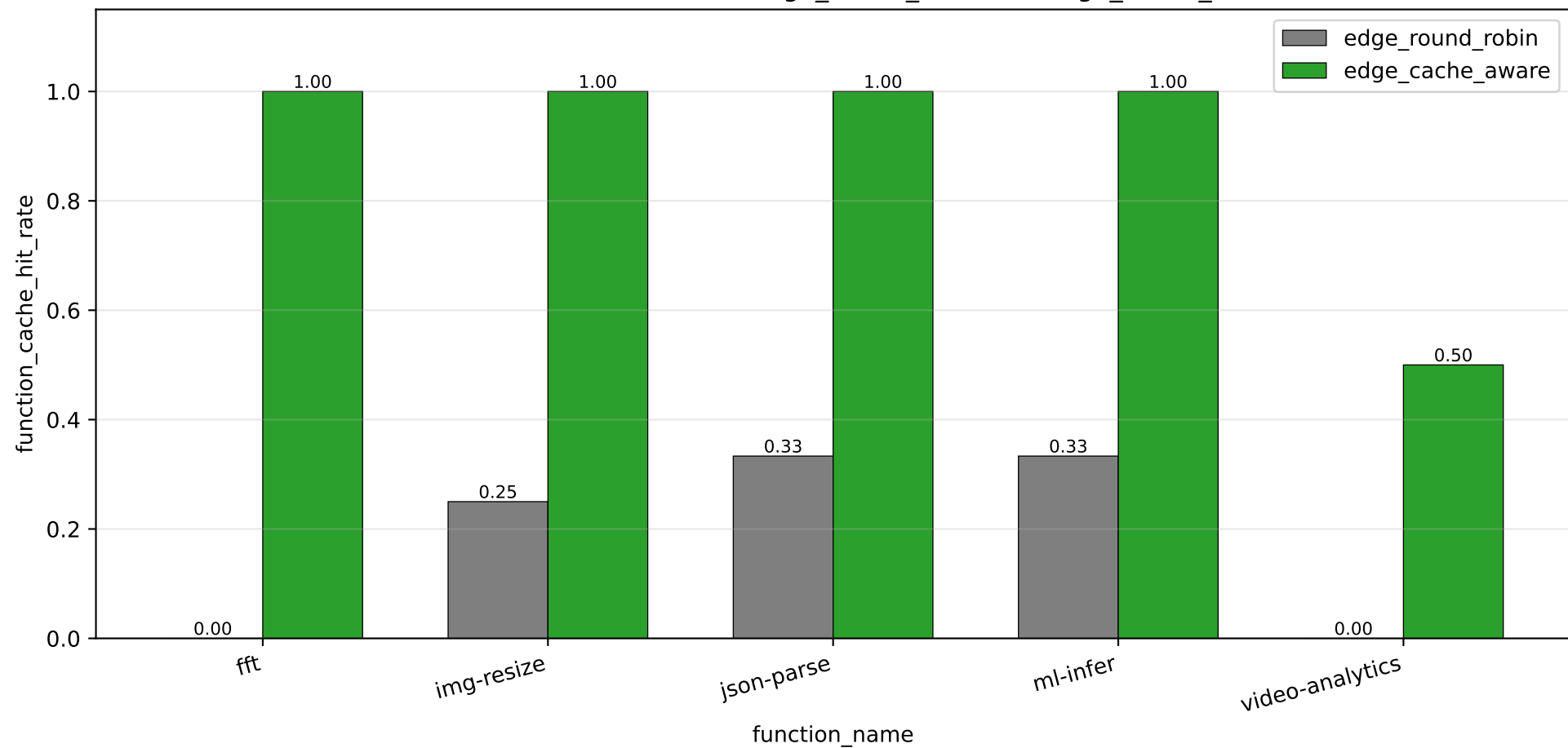
Per-function cache hit rate: edge_cache_aware vs edge_round_robin
