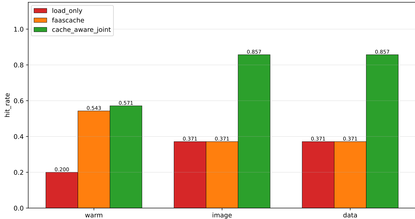
Thesis: three cache dimension hit rates by case
