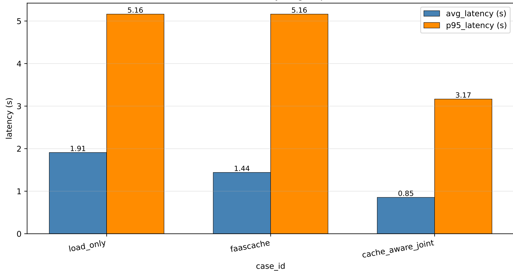
Per-case latency: avg vs p95
