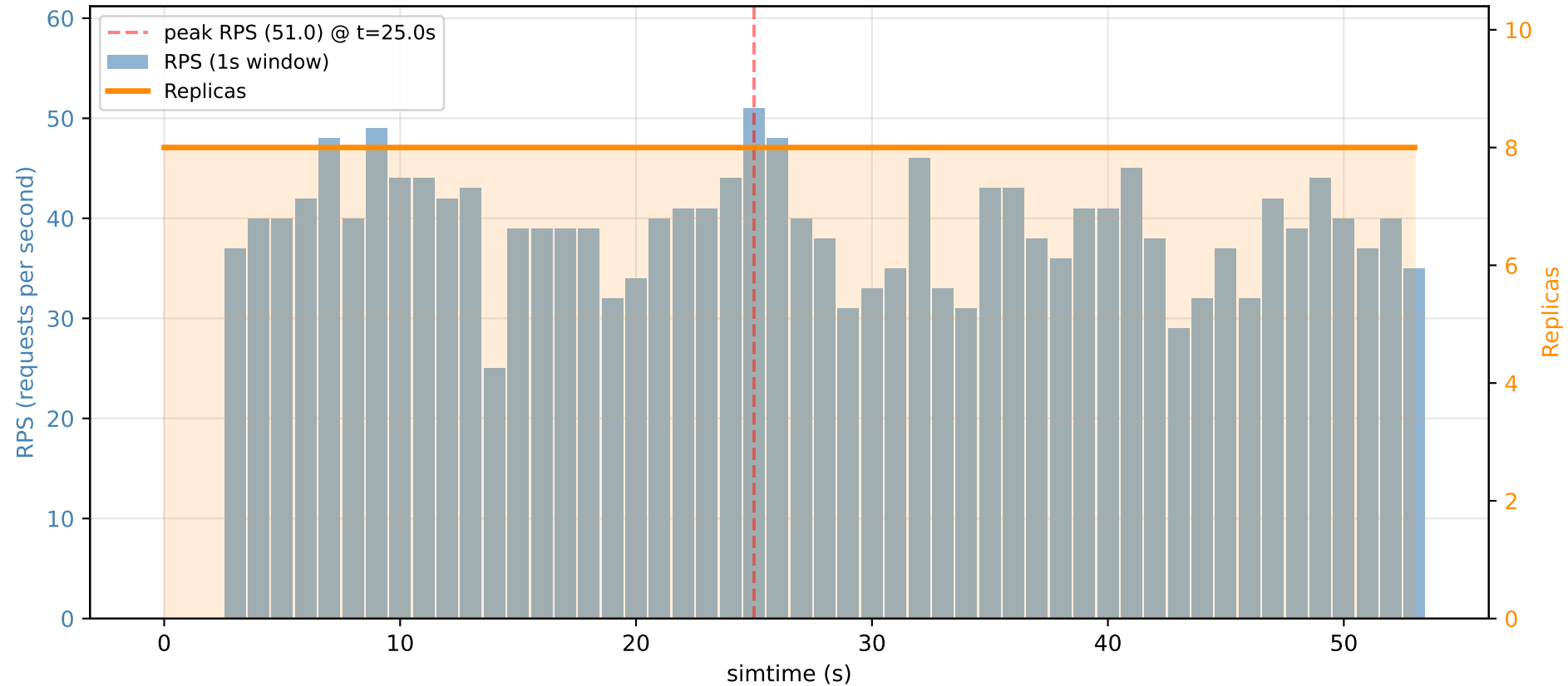
Autoscaling behavior under constant 40 RPS load (RPS vs Replicas timeline)
