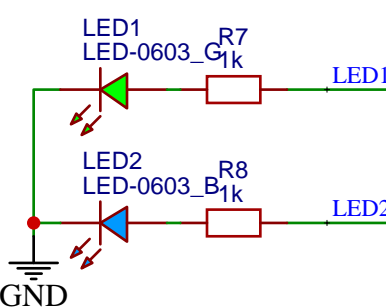
LED
