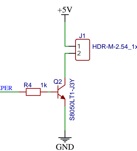
BEEPER
