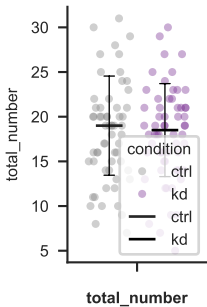
total_number
