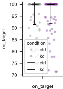
on_target
